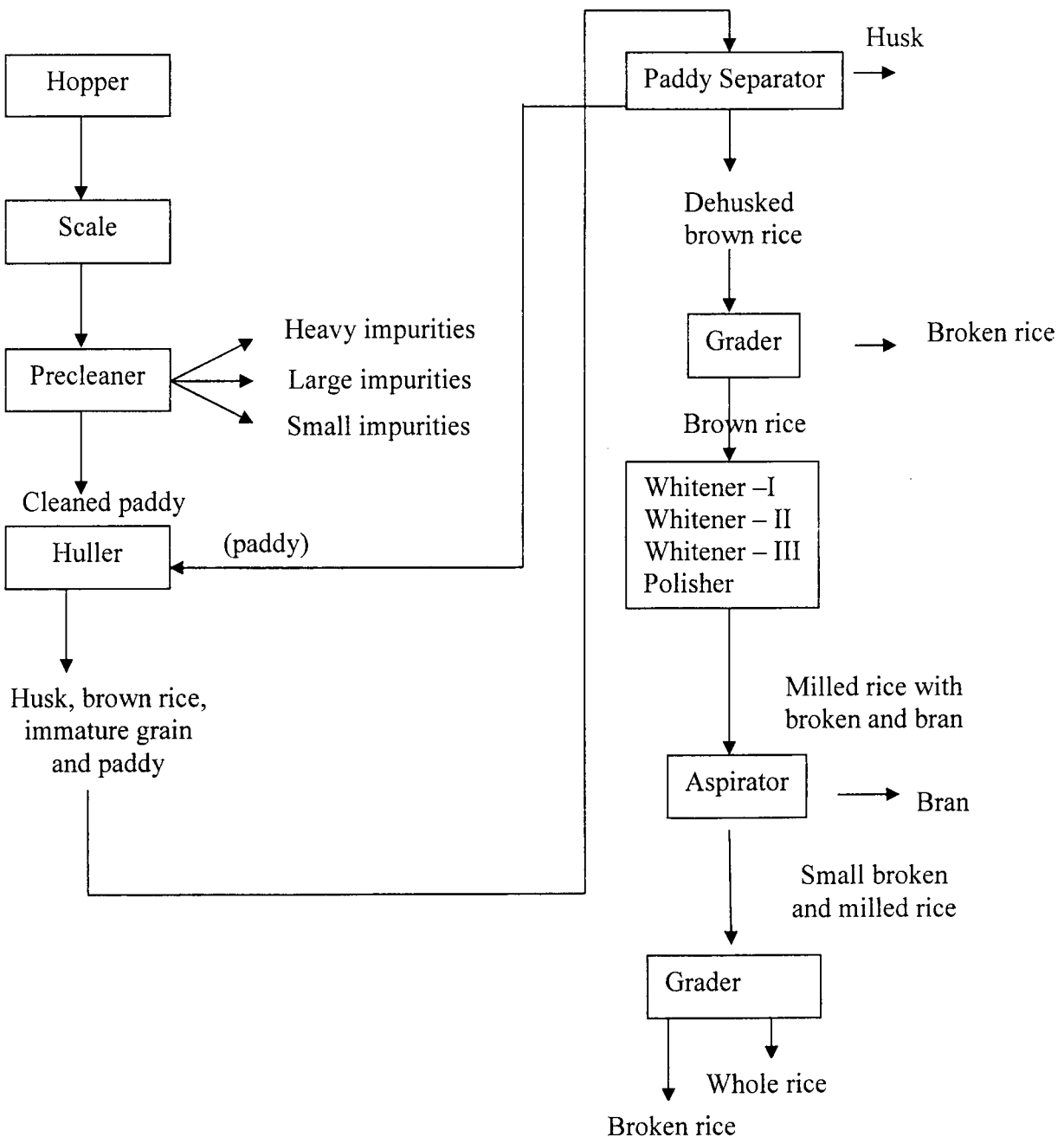
Fig. 11: Modern Milling System
